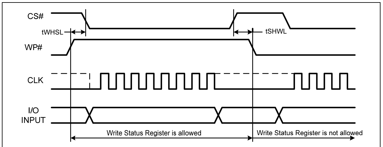
Figure 88 WP# Timing
