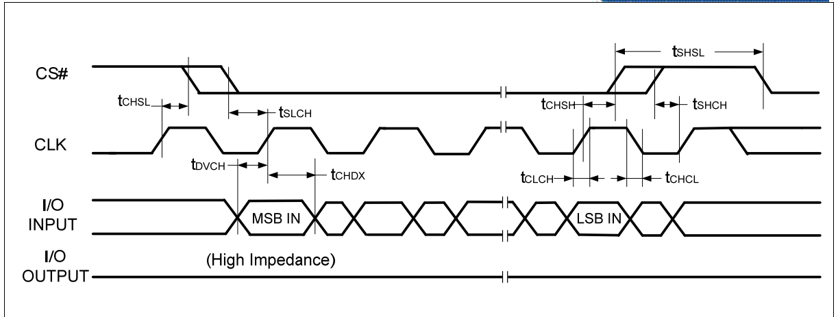
Figure 86 Serial Input Timing
