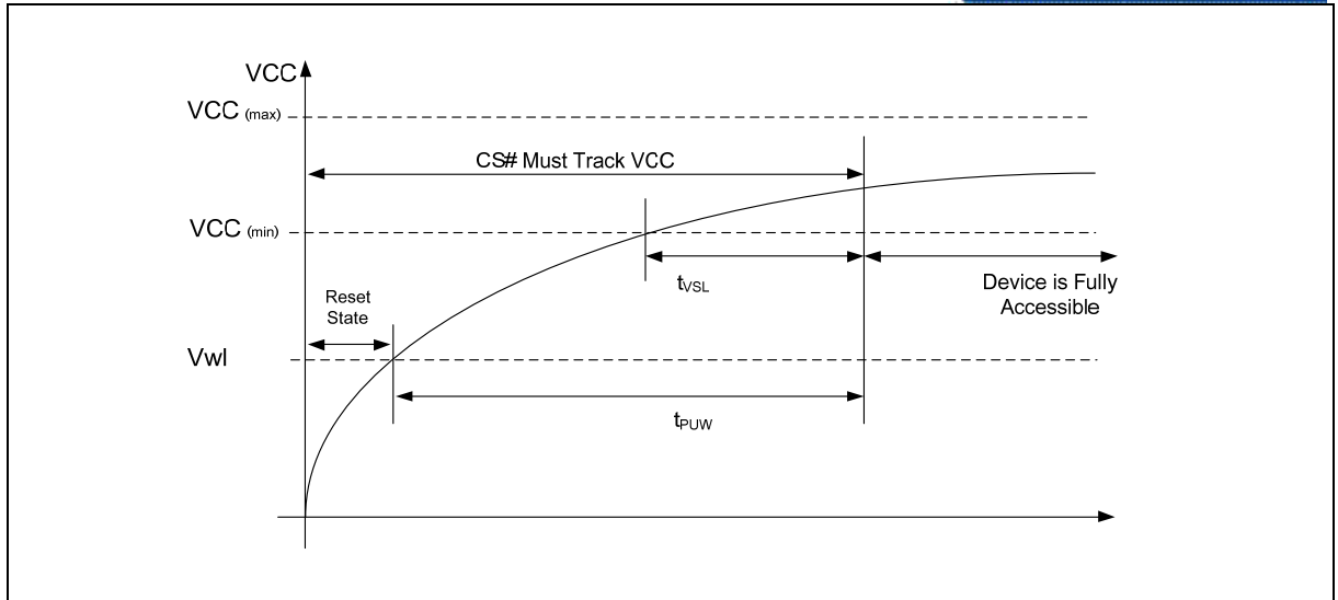
Figure 83 Power-up Timing
