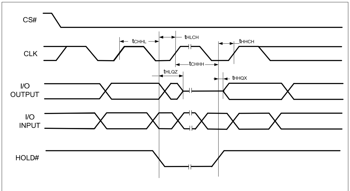
Figure 87 Hold Timing
