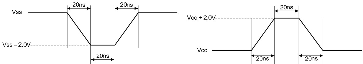
Figure 81 Maximum Negative Overshoot Waveform Figure 82 Maximum Positive Overshoot Waveform
