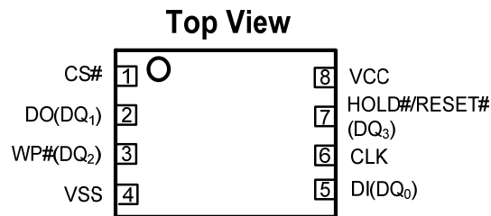
Figure 2 FM25W128 pad assignments, 8-pad TDFN(6x5mm)
