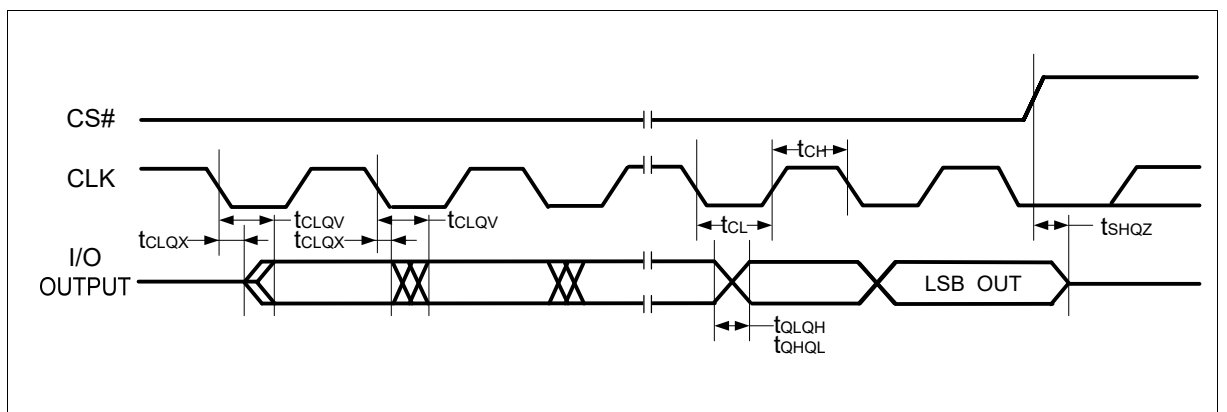
Figure 85 Serial Output Timing
